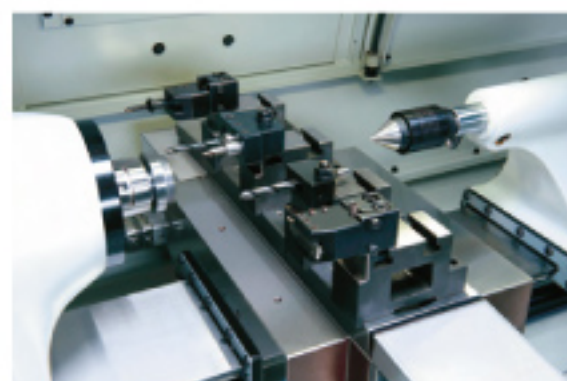
Multiple "single" gang tool blocks each holding a single tool holder.
