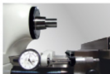
Indicator Carriage Stop
